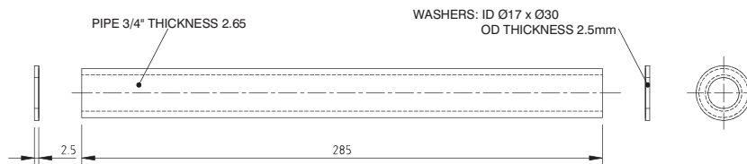
Figure 2. 80L Distance Pipe Dimensions
