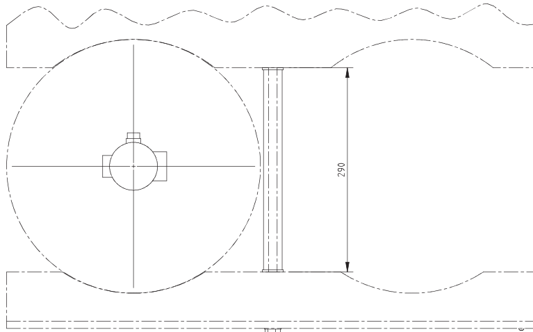
Figure 3. 140L Distance Pipe Dimensions
